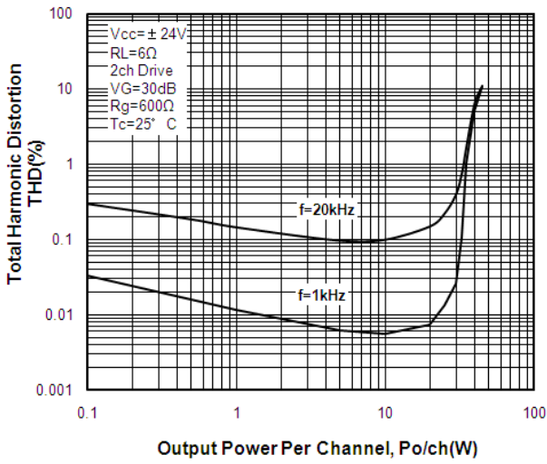
THD-Po STK433-040N-E
